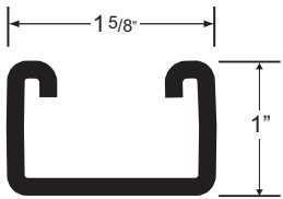
M-12 Channel
