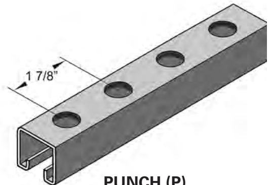
PUNCH (P)
