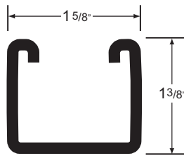
B-12 Channel
