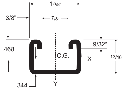
C-12
