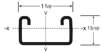
C-14 Channel
