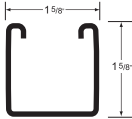
A-14 Channel
