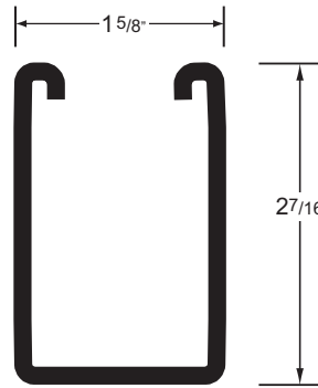
D-12 Channel
